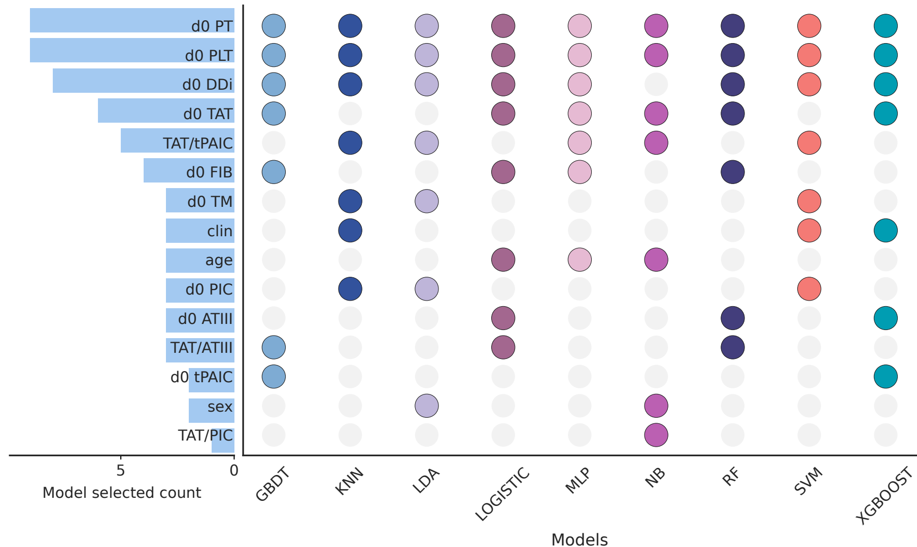
Feature selection dot matrix across models
